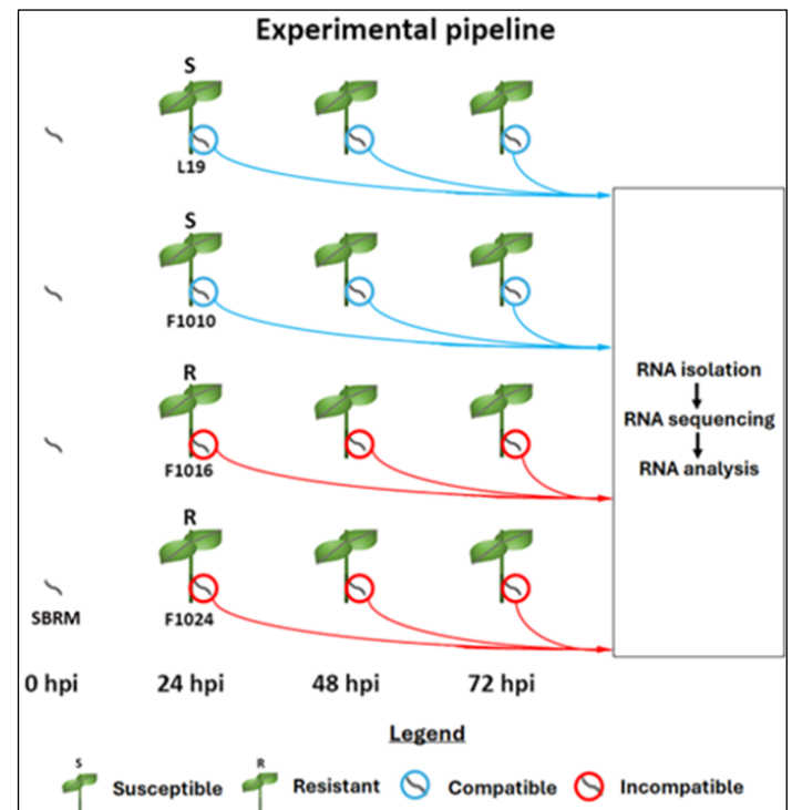
Figure 1: Experimental Pipeline
